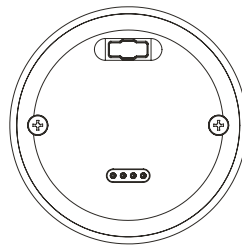
ProMount Hardwired Wall Mount Requires 2-3/8" hole saw.
